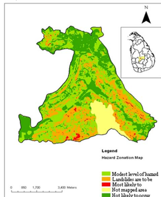
Figure 2. Existing LHZ map
