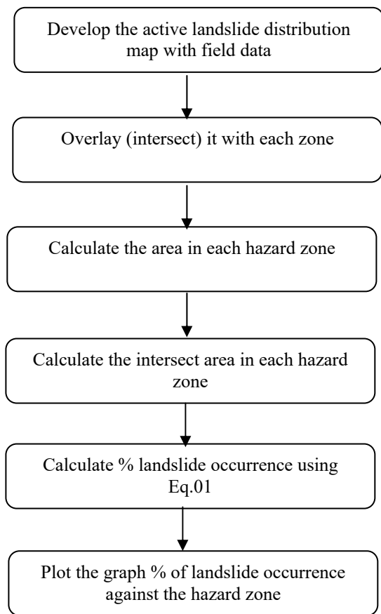
Figure 3. Validating procedure of existing LHZ map
